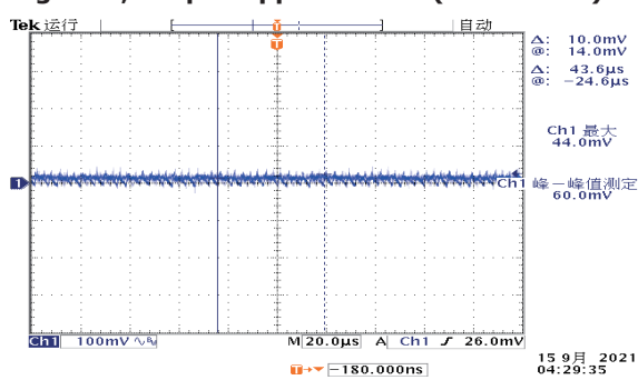
Figure 7, Output ripple & noise (Iout = 20A)
