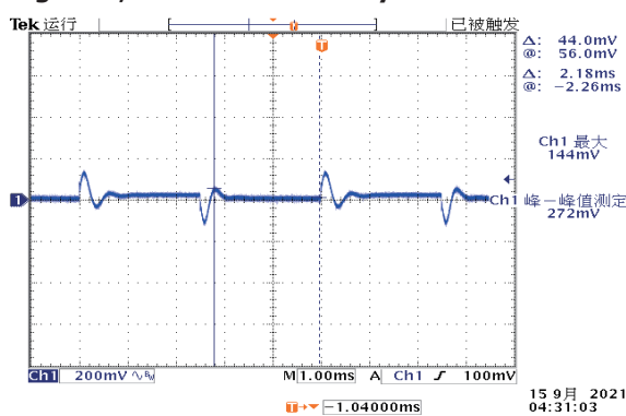
Figure 5, 50% - 75% load dynamic
