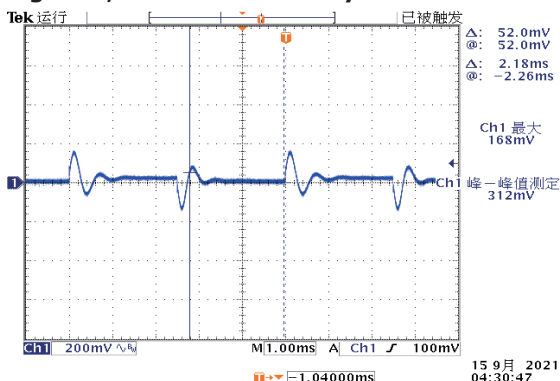
Figure 4, 25% - 50% load dynamic
